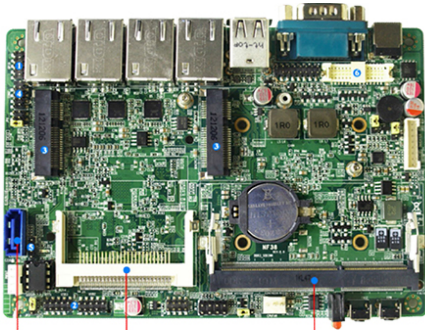
1 * Serial ATAII 3Gb/s connector CF card reader socket (can support both CF card & CF SATA card) 1 * DDR3 667/800MHz Single CH SO-DIMM up to 2GB
