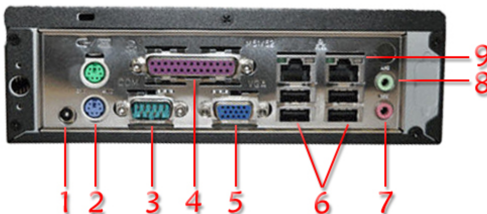
6. 4x USB 2.0
