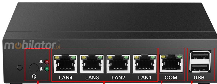
Power On/Off 4x LAN COM 2x USB 2.0
